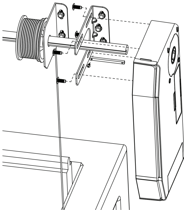
Jack shaft with keyway installation
