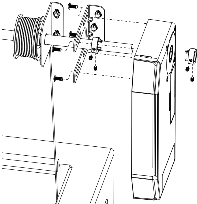
Jack shaft keyless installation
